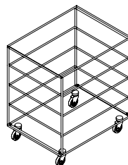
Comp. fix 8/a 58 x 45 x h 66
