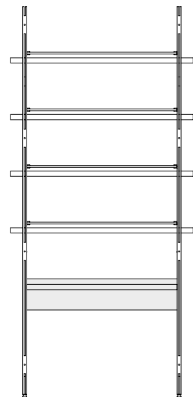
Comp. 215 121,4 x 63 x H 260 cm 2xM2 + 4xR2 + 1S1
