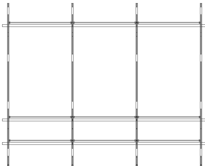
Comp. 407 326,8 x 37 x H 260 cm 4xM2 + 9xR2
